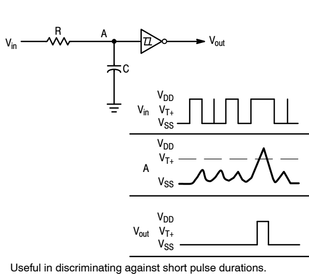
Figure 6. Integrator
