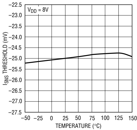
I_{SNS} Threshold vs Temperature
