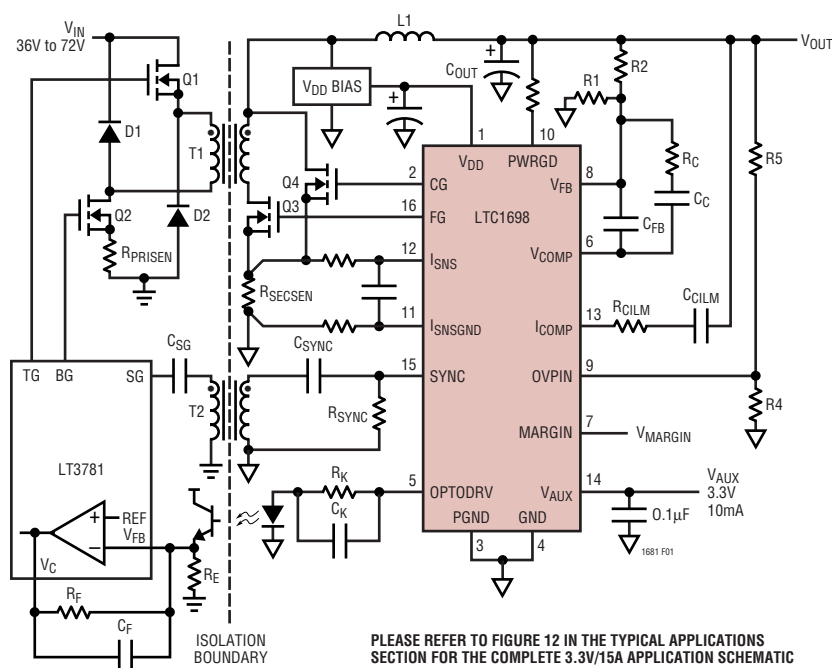
Figure 1. Simplified 2-Transistor Isolated Forward Converter
