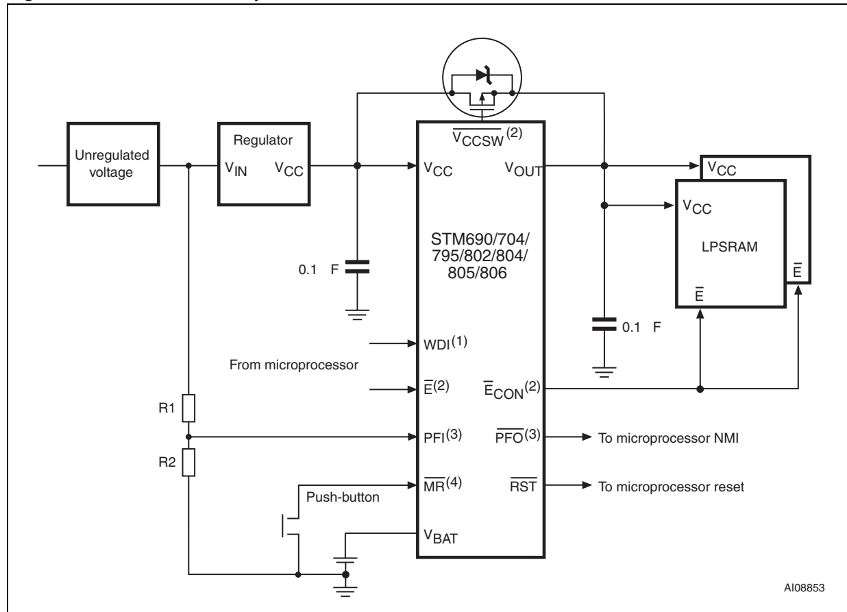
Figure 10. Hardware hookup
