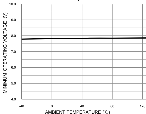
Minimum Operating Voltage vs. Ambient Temperature
