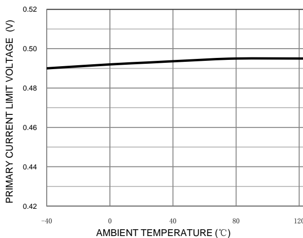
Current Limit Voltage vs. Ambient Temperature
