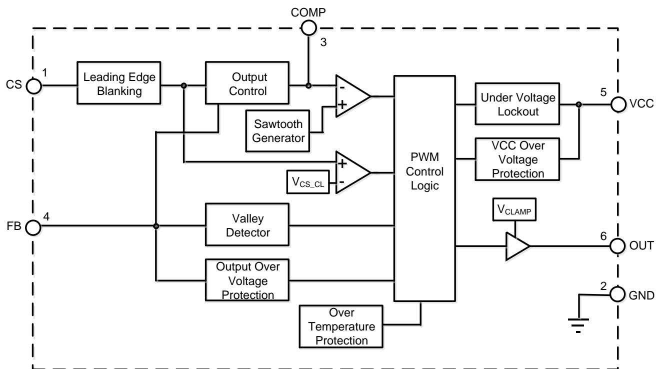
Figure 3. AL1788 Controller Functional Block Diagram
