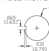
15/32 INCH BUSHING
