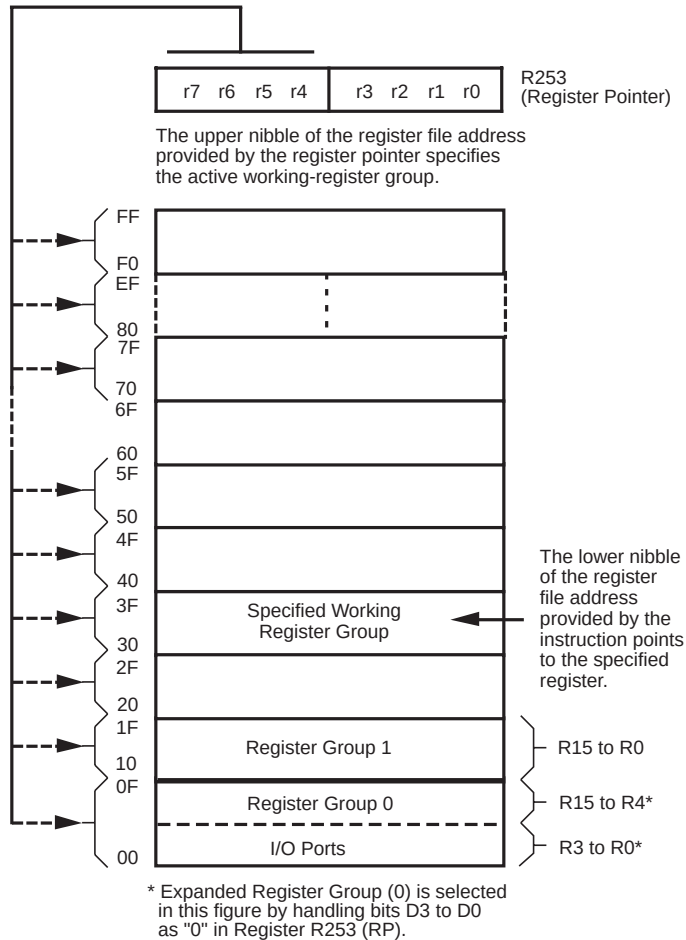
Figure 21. Register Pointer
