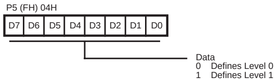
Figure 48. Port 5 Data Register (F)04: (Read/Write)
