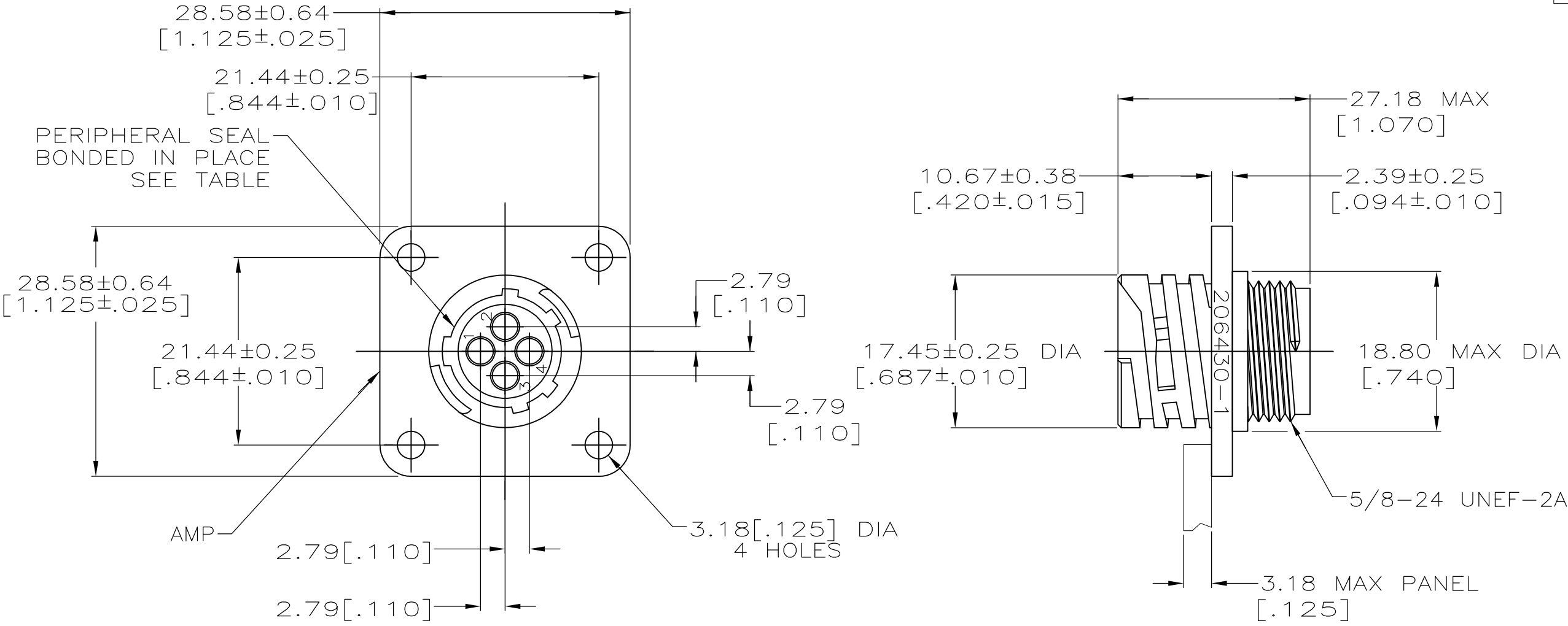
DETAIL A
