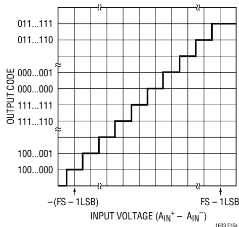
Figure 15a. LTC1603 Transfer Characteristics
