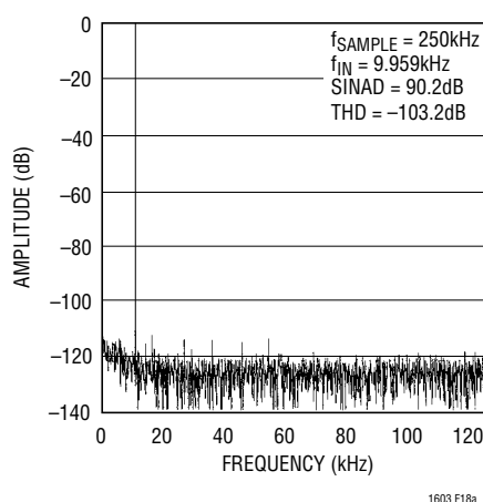
Figure 18a. This FFT of the LTC1603's Conversion of a Full-Scale 10kHz Sine Wave Shows Outstanding Response with a Very Low Noise Floor When Sampling at 250ksps
