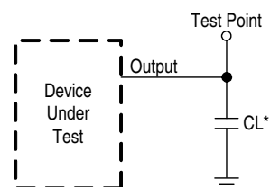
Figure 12. Test Circuit
