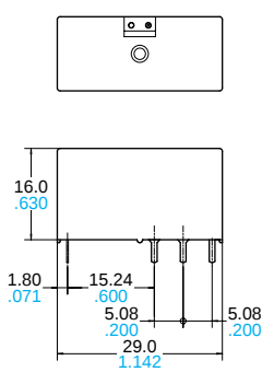
1 coil latching type
