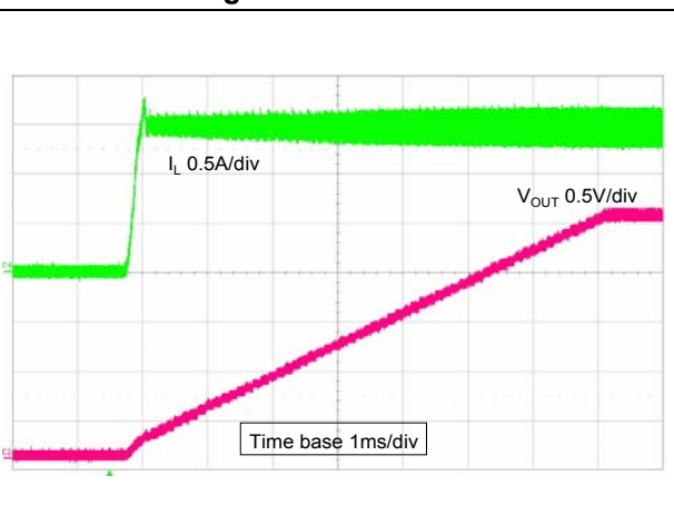
Figure 30. Soft-start
