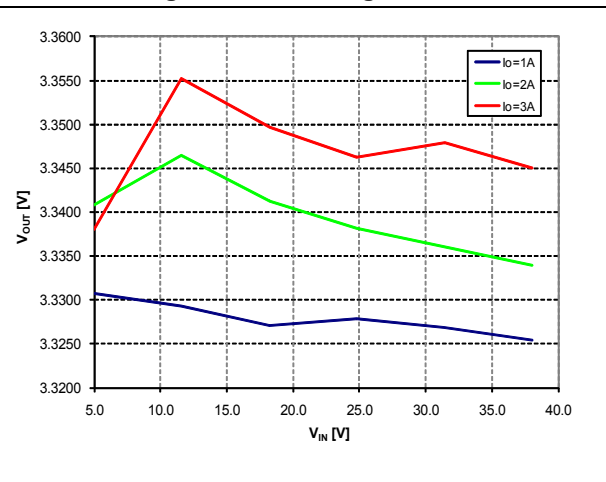
Figure 28. Line regulation
