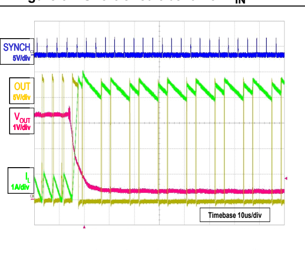
Figure 32. Short-circuit behavior V_{IN} = 24 V
