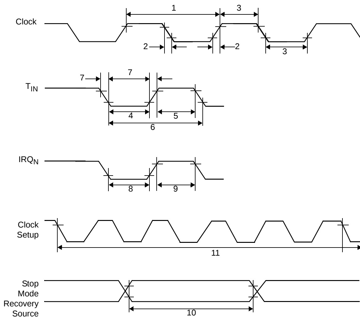
Figure 5. Additional Timing
