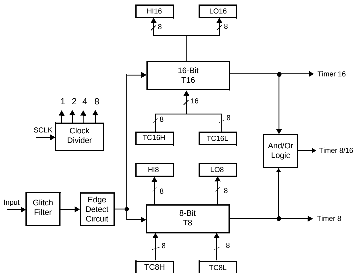
Figure 1. Counter/Timers Diagram
