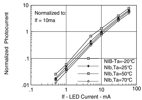
Fig. 10 Normalized Photocurrent vs. LED Current
