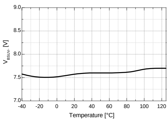
Figure 19. V BS UVLO- vs. Temp.
