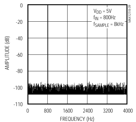
FFT PLOT
