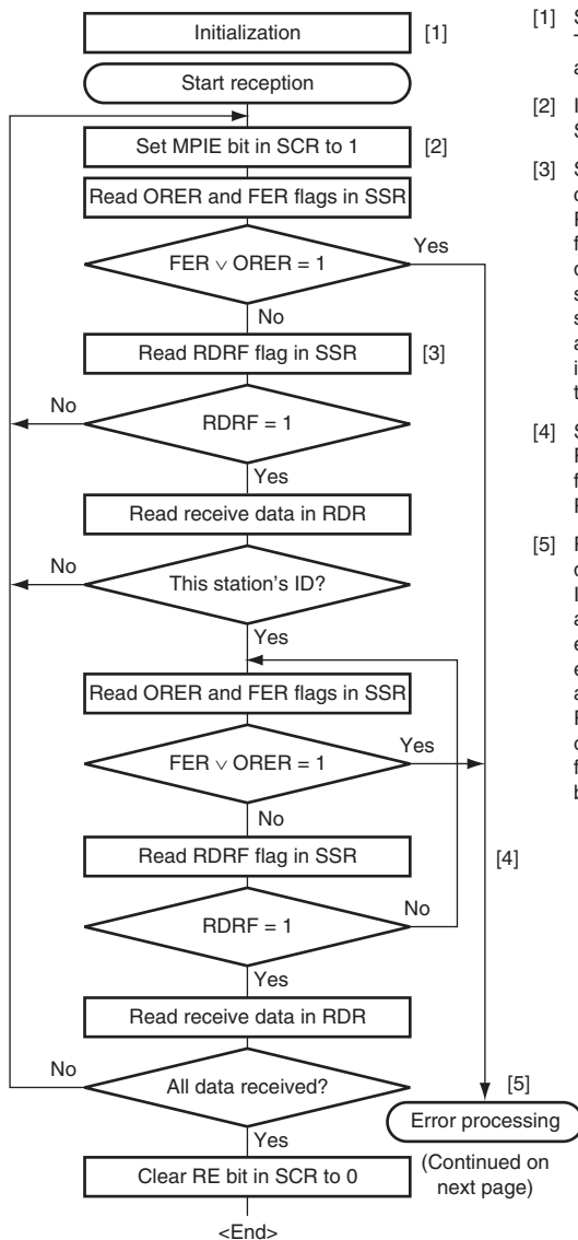
Figure 19.16 Sample Multiprocessor Serial Reception Flowchart (1)
