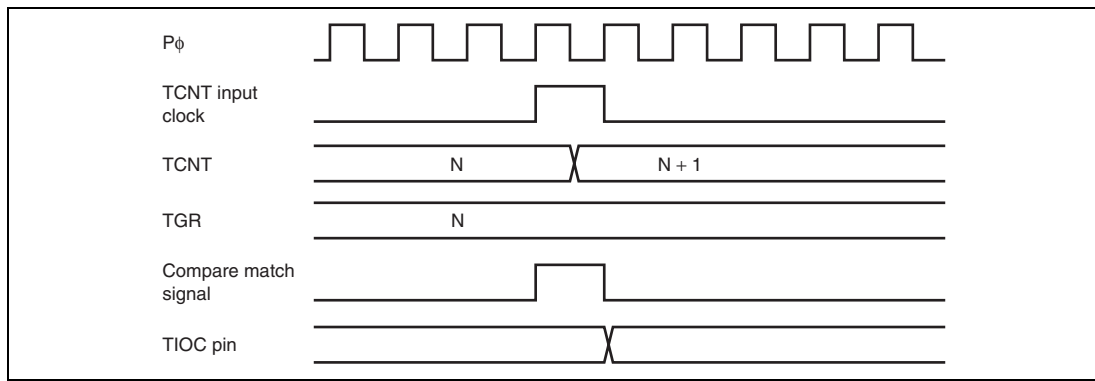
Figure 14.32 Output Compare Output Timing
