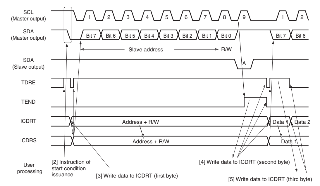
Figure 21.5 Master Transmit Mode Operation Timing 1
