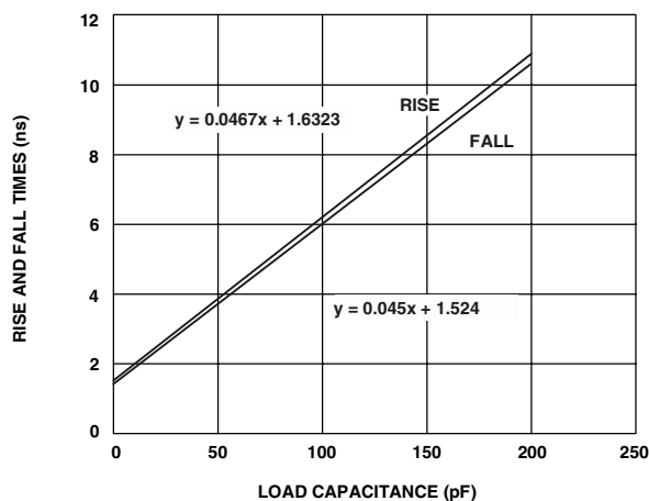
Figure 39. Typical Output Rise/Fall Time (20%-80%, V_{DDEXT} = \text{Max} )
