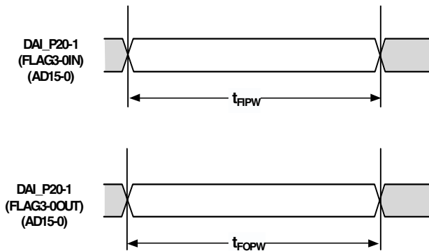
Figure 16. Flags
