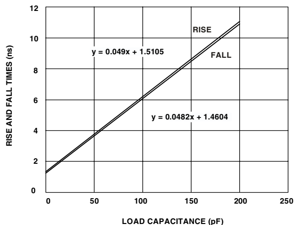
Figure 40. Typical Output Fall Time (20%-80%, V_{DDEXT} = \text{Min} )
