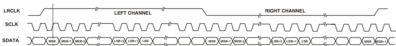
Figure 29. Left-Justified Mode
