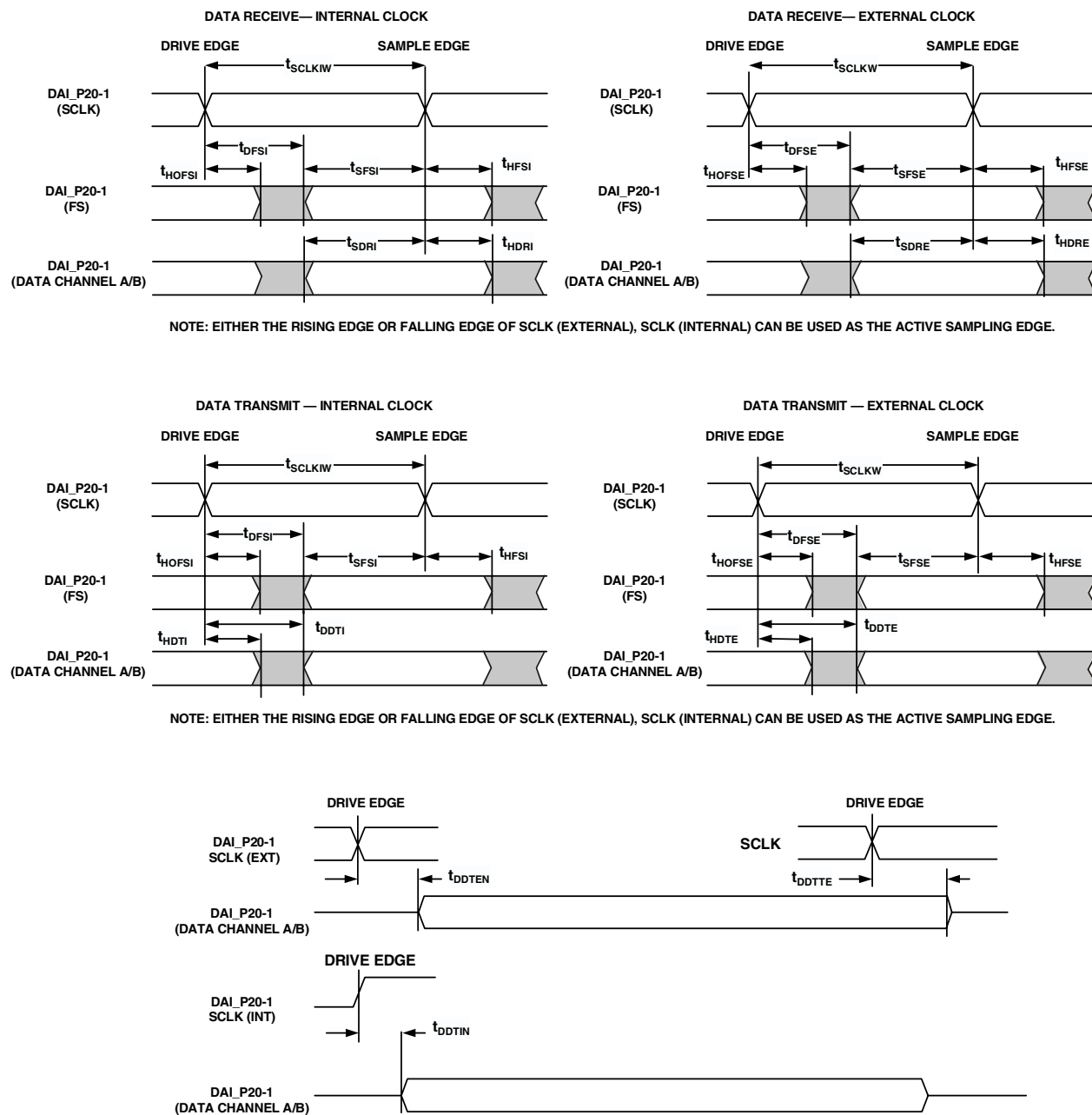
Figure 22. Serial Ports
