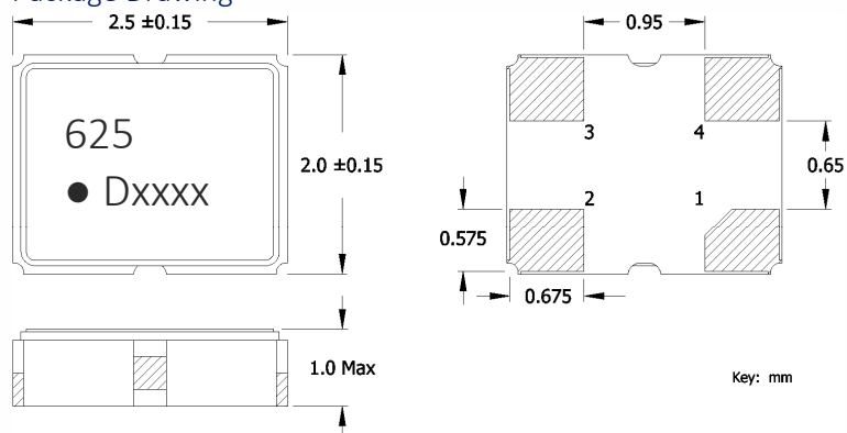
Package Drawing
