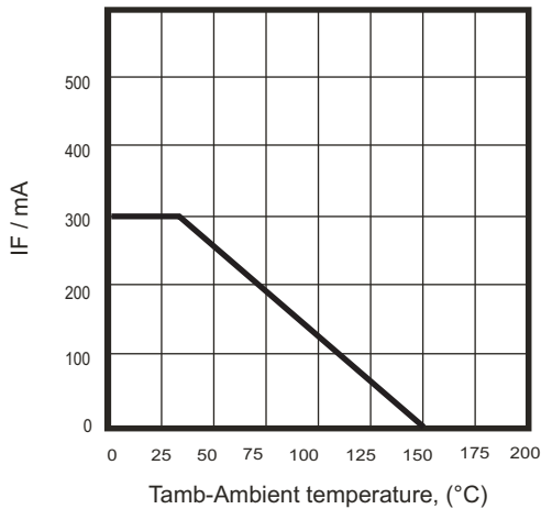
Fig.3 - Forward Current De-rating
