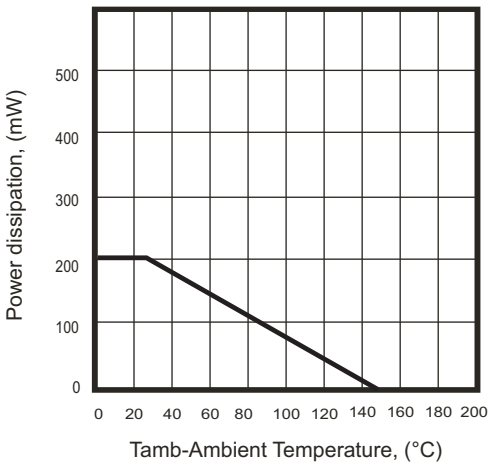
Fig.2 - Power De-rating
