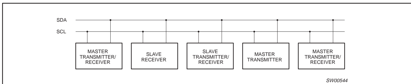
Figure 17. System configuration
