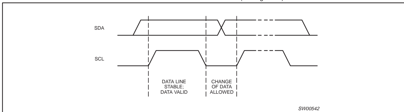
Figure 15. Bit transfer
