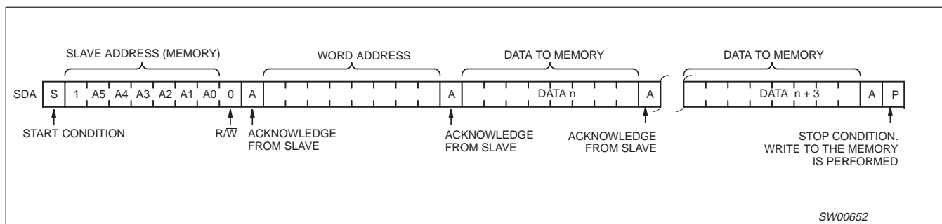
Figure 11. Page Write
