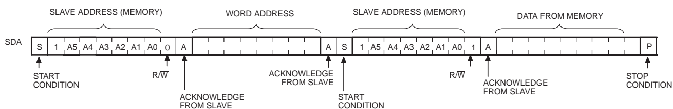
Figure 13. Random Read
