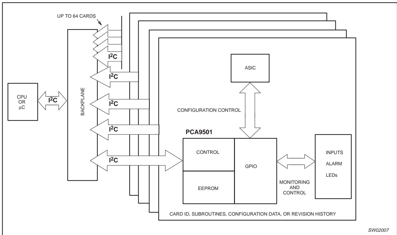
Figure 19. Typical application
