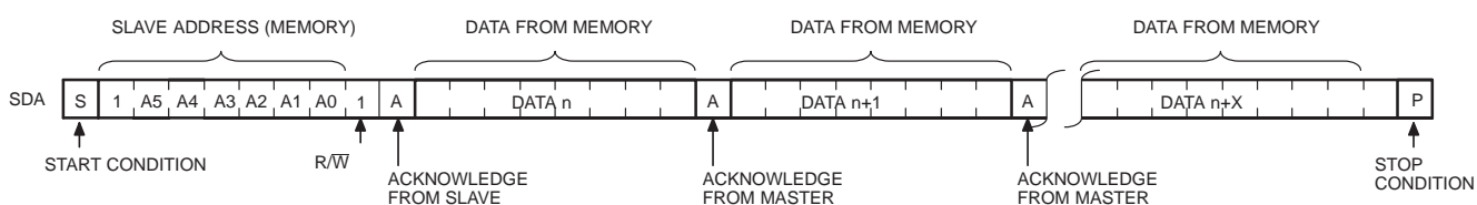
Figure 14. Sequential Read
