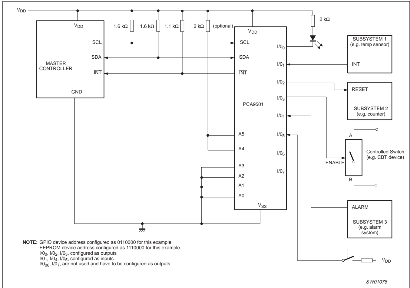
Figure 20. Typical application
