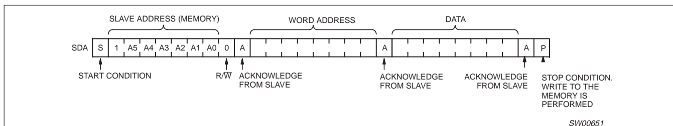
Figure 10. Byte write
