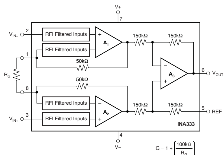
Simplified Schematic
