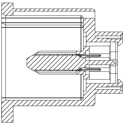
SECT B-B
