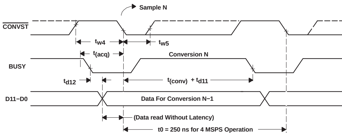
Figure 7. Back-To-Back Operation With \overline{CS} and \overline{RD} Low
