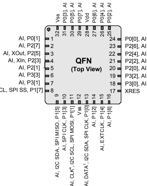
Figure 5. CY8C20436, CY8C20446, CY8C20466 PSoC Device
