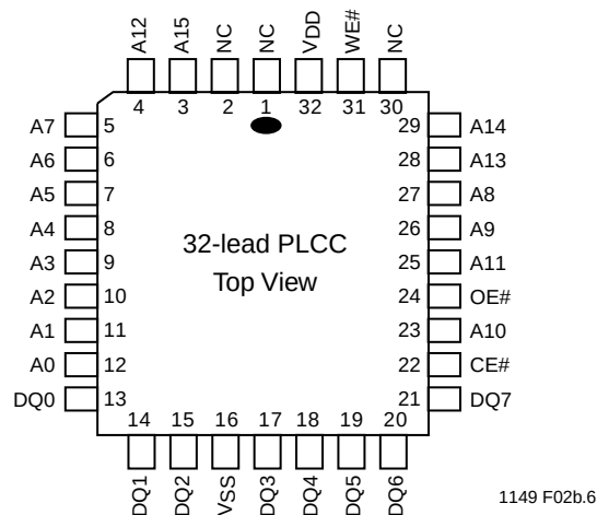
FIGURE 1: PIN ASSIGNMENTS FOR 32-LEAD PLCC
