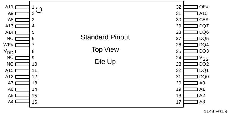
FIGURE 2: PIN ASSIGNMENTS FOR 32-LEAD TSOP (8MM X 14MM)
