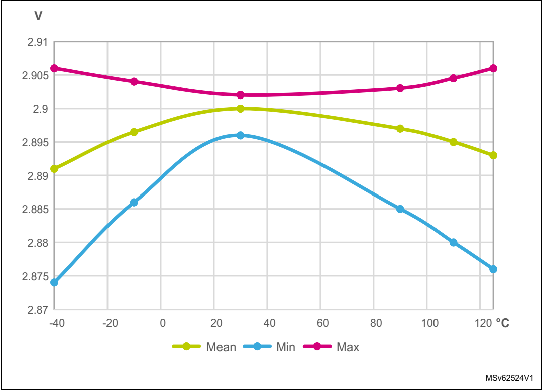
Figure 34. V_{\text{REFOUT}} TEMP in case VRS = 10
