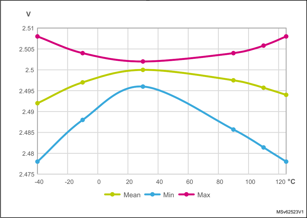
Figure 33. V_{\text{REFOUT}} TEMP in case VRS = 01
