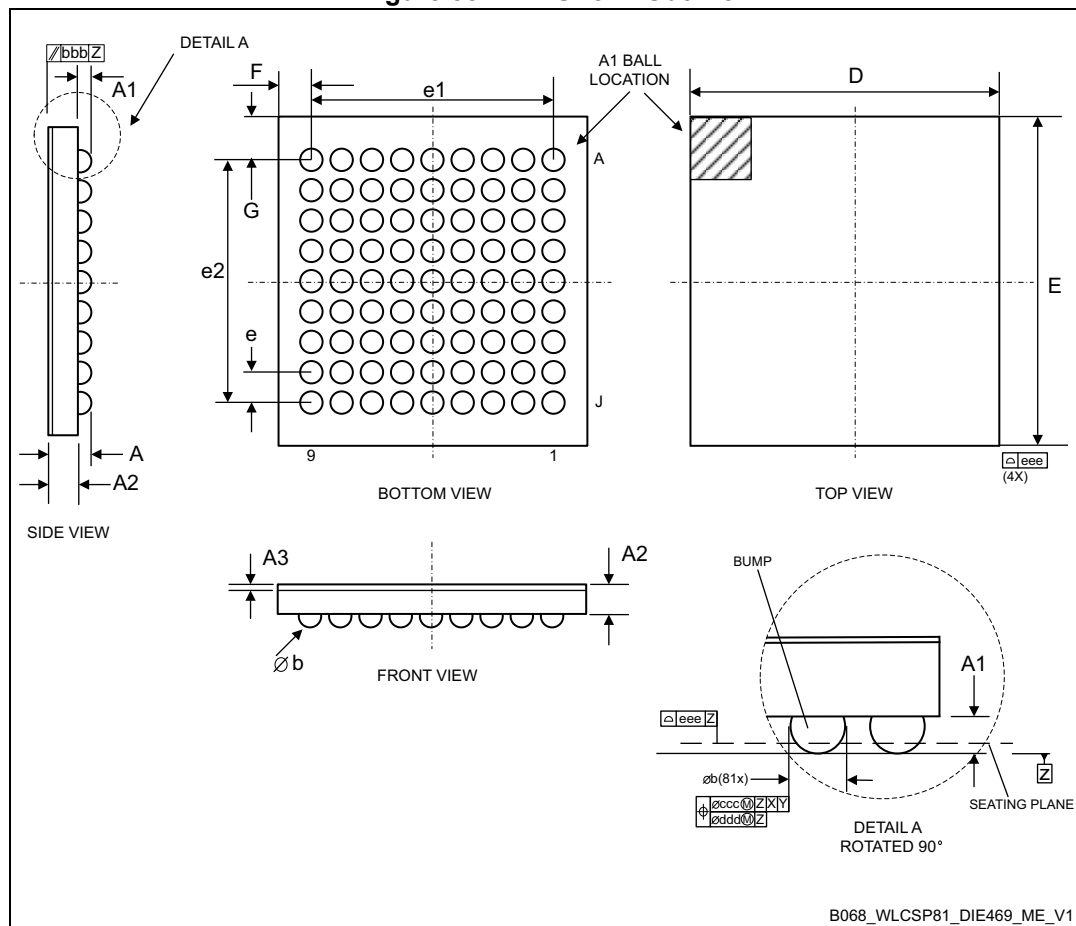
Figure 55. WLCSP81 - Outline
