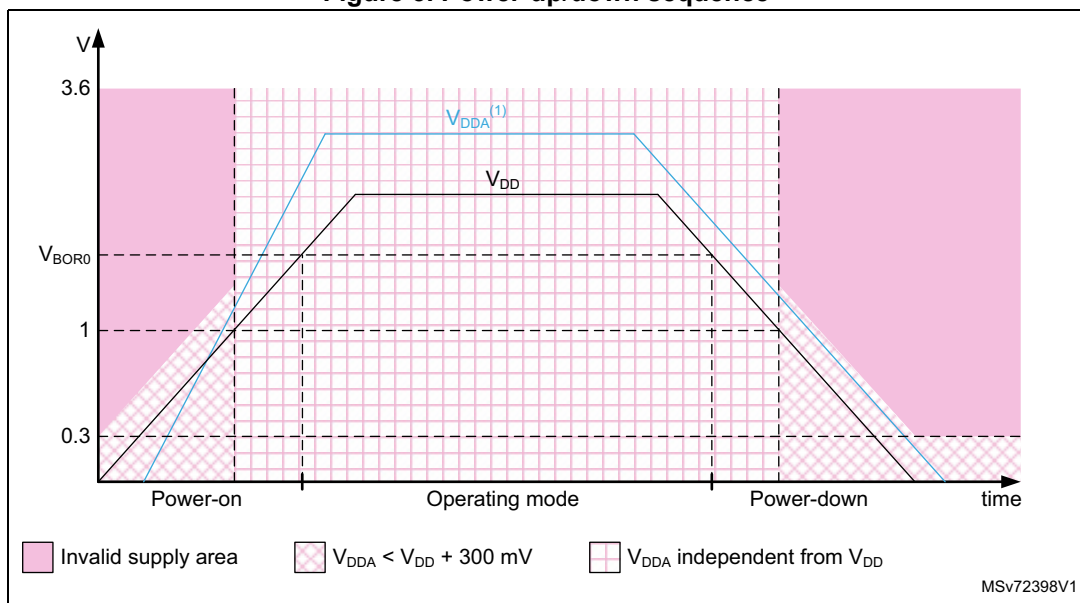
Figure 3. Power-up/down sequence
