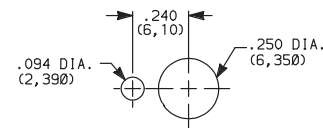
Without Locking Ring
