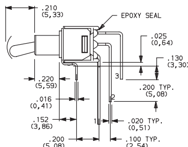
T102 Models: Omit terminal 2
