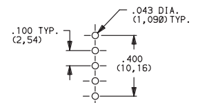
T102 Models: Omit center hole.
