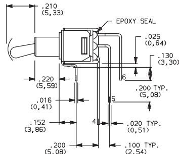
T102 Models: Omit terminal 2
