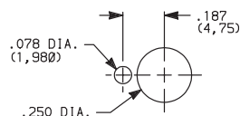
With Small Locking Ring
