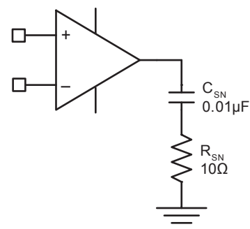
FIGURE 5. R-C Snubber
