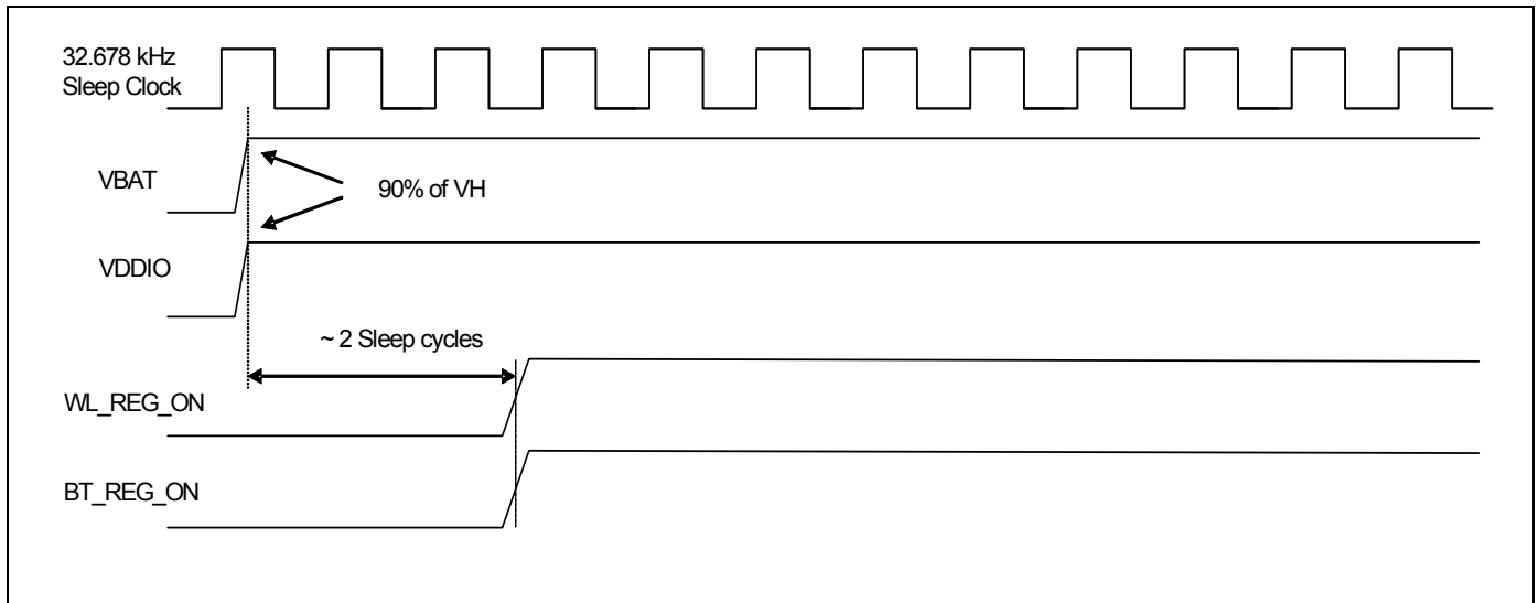
Figure 38. WLAN = ON, Bluetooth = ON
