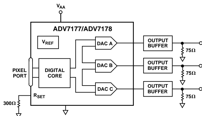
Figure 67. Output DAC Buffering Configuration
