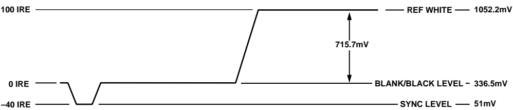
Figure 52. NTSC RGB Video Levels
