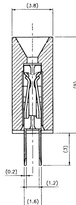
SECTION U-U
