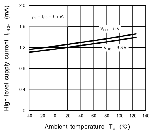
Fig. 12.2.8 I_{DDH} - T_a
