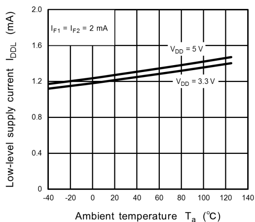
Fig. 12.2.7 I_{DDL} - T_a
