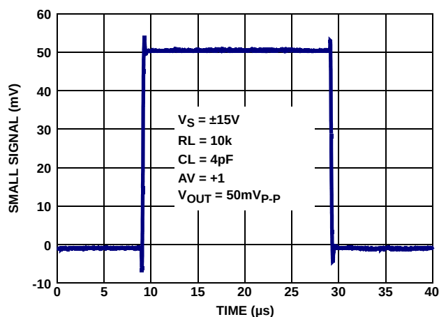
FIGURE 5. SMALL SIGNAL TRANSIENT RESPONSE, V_S = \pm 5V, \pm 15V
