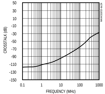
MAX4310/MAX4313 ALL-HOSTILE CROSSTALK vs. FREQUENCY
