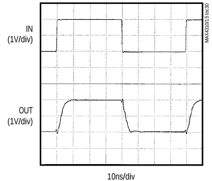
MAX4310 LARGE-SIGNAL PULSE RESPONSE
