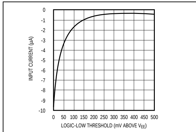
Figure 4. Logic-Low Input Current vs. V_{IL} with 10kΩ Series Resistor
