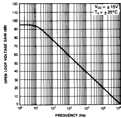
Figure 1. Open Loop Frequency Response
