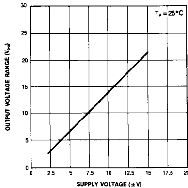
Figure 3. Output Swing
