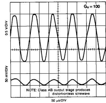
Figure 2. Wave Response
