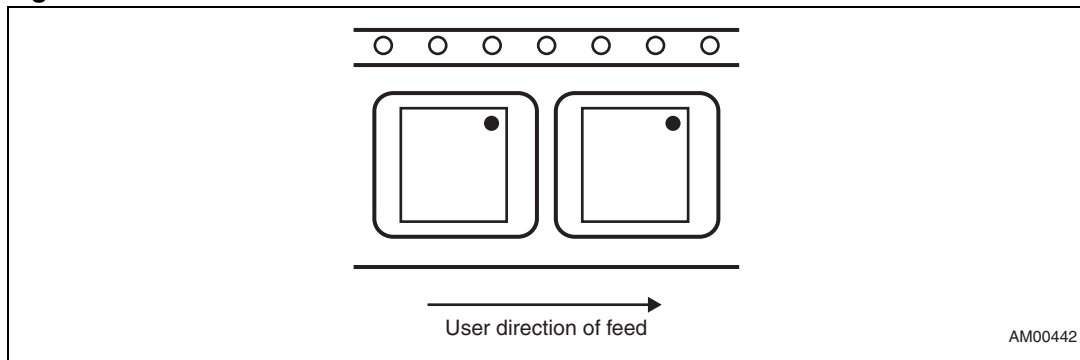
Figure 17. Pin 1 orientation
