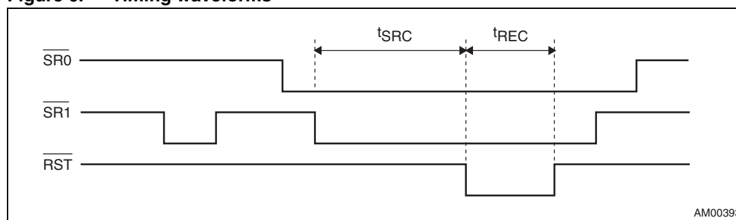
Figure 6. Timing waveforms
