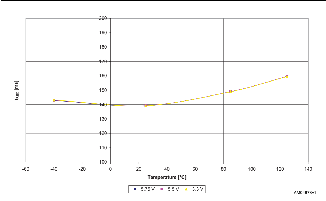
Figure 9. Reset timeout period ( t_{REC} ) vs. temperature, C_{tREC} = 0.01 \mu F
