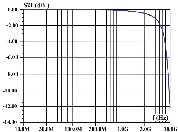
Figure 4. S21 (dB) attenuation
