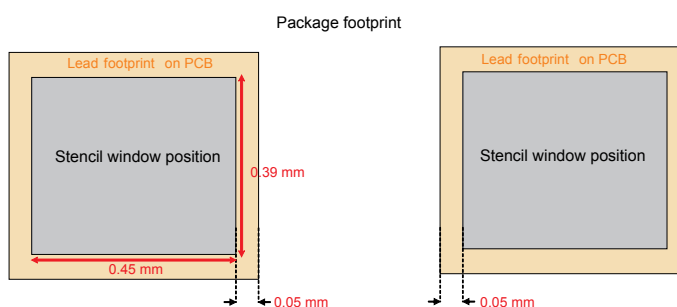
Figure 13. Recommended stencil window position in mm
