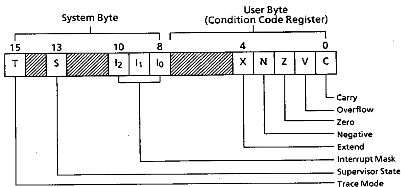
Figure 1.3 Status Register
