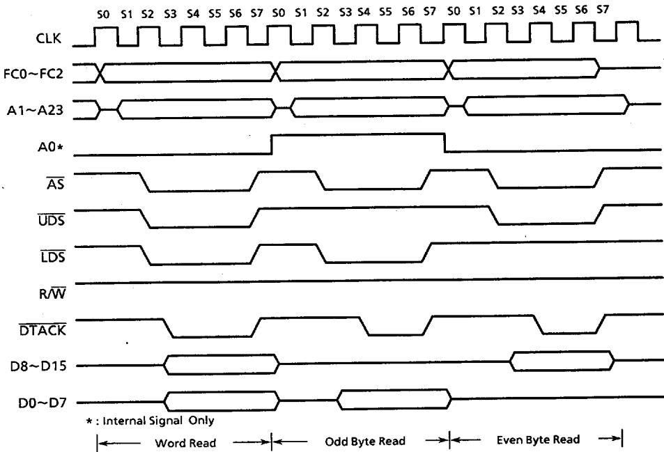
Figure 4.5 Word and Byte Read Cycle Timing Diagram
