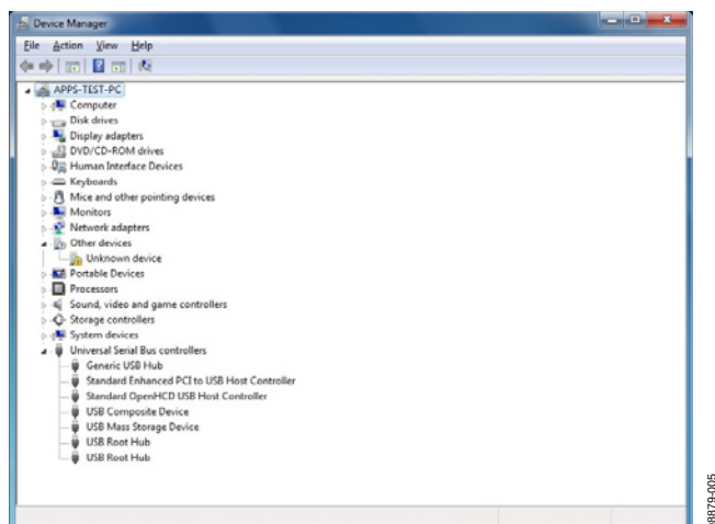
Figure 5. Device Manager
