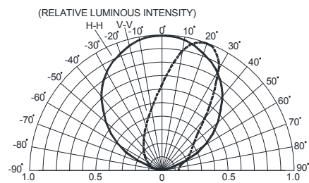
FIG.6b RED & BLUE&GREEN FAR FIELD PATTERN
