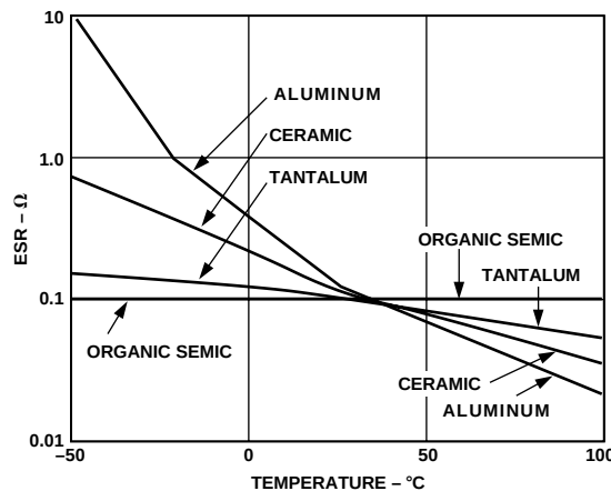
Figure 19. ESR vs. Temperature
