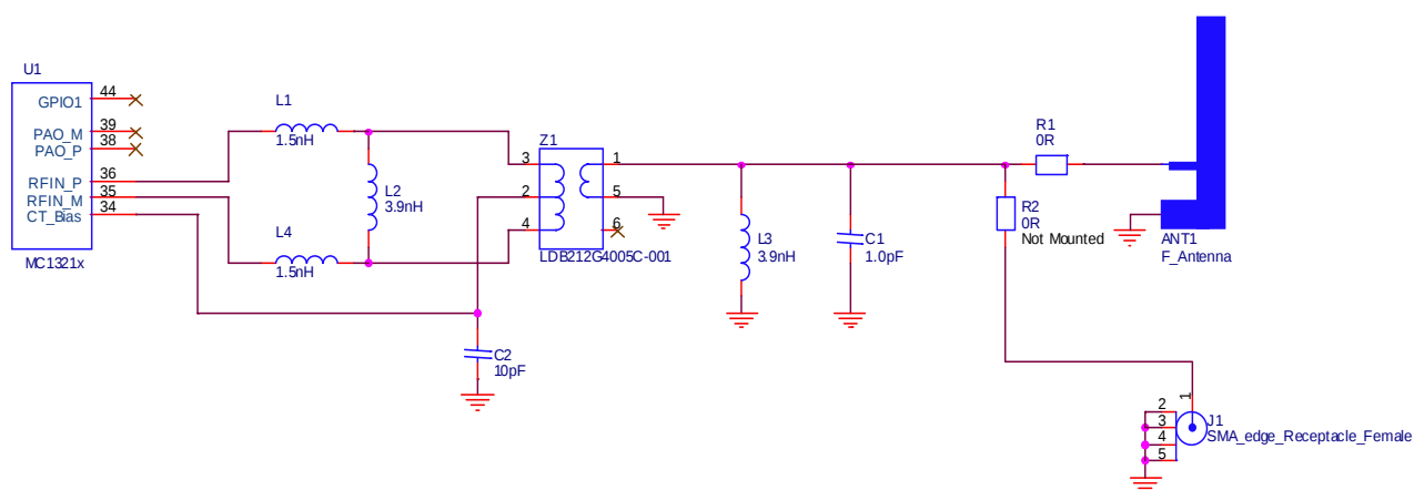
Figure 35. RF Single Port Application with an F-Antenna
