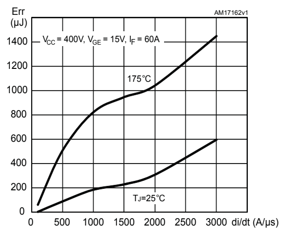
Figure 24. Reverse recovery current vs. energy current slope
