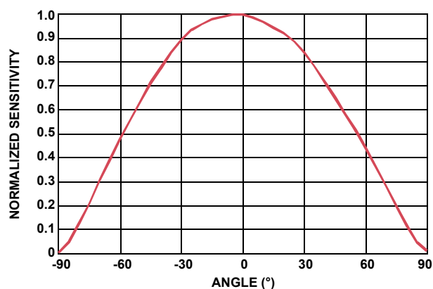
FIGURE 12. ANGULAR SENSITIVITY
