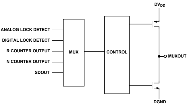
Figure 21. MUXOUT Circuit
