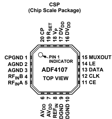
Figure 4. ADF4107 Chip Scale Package
