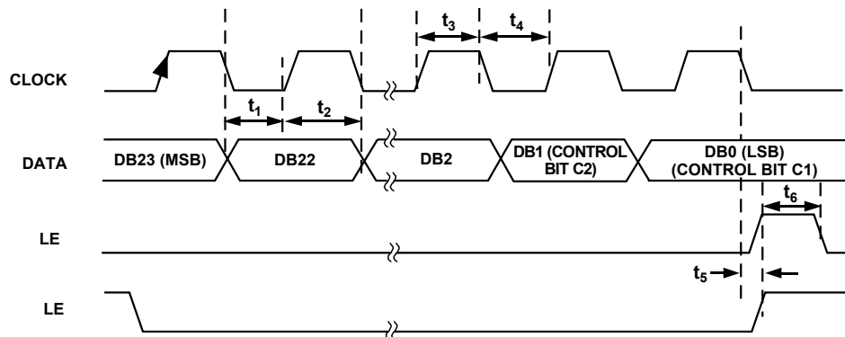
Figure 2. Timing Diagram
