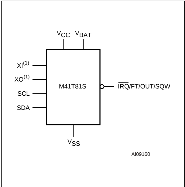
Figure 2. Logic Diagram
