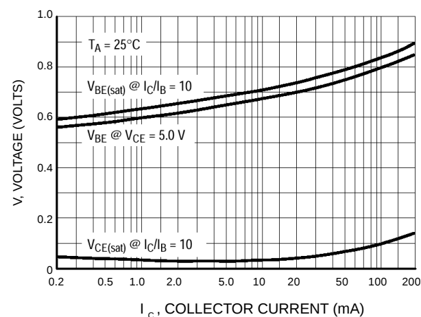
Figure 8. "On" Voltage
