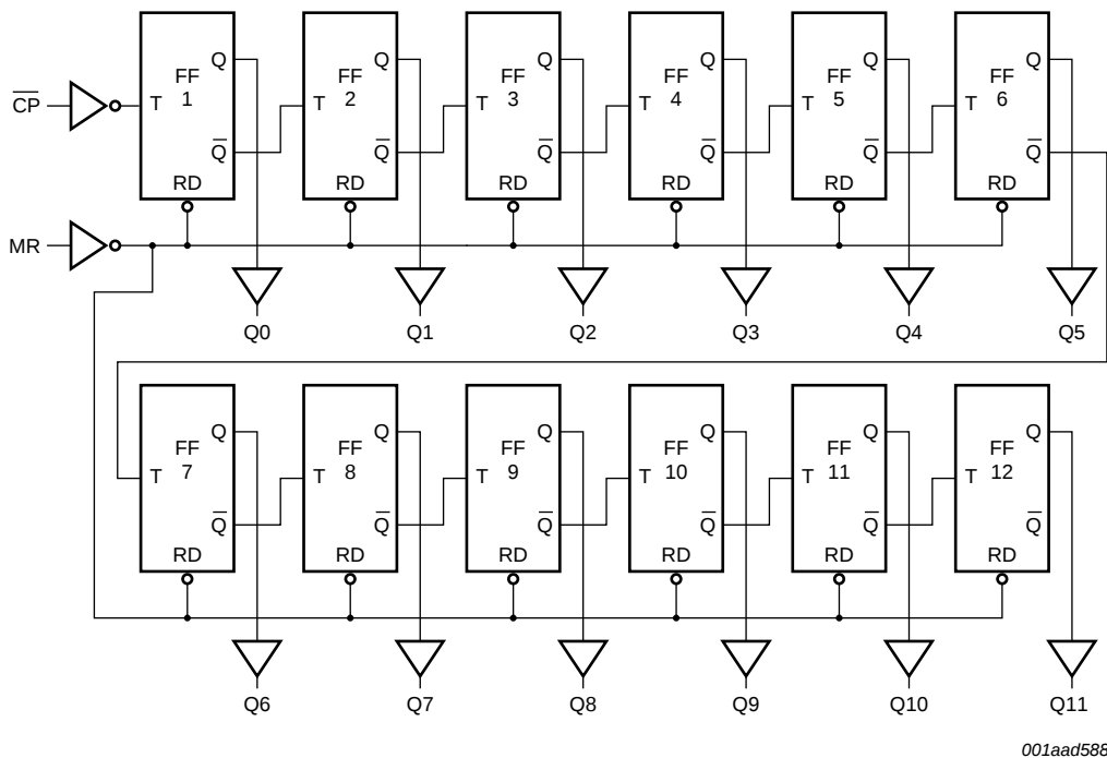
Fig 4. Logic diagram
