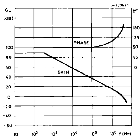
Figure 3. Open loop frequency response.
