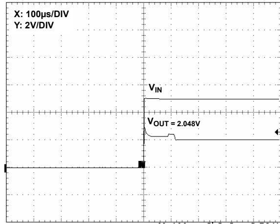
FIGURE 24. TURN-ON TIME
