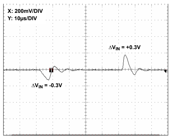
FIGURE 10. LINE TRANSIENT RESPONSE, 0.001μF LOAD CAPACITANCE
